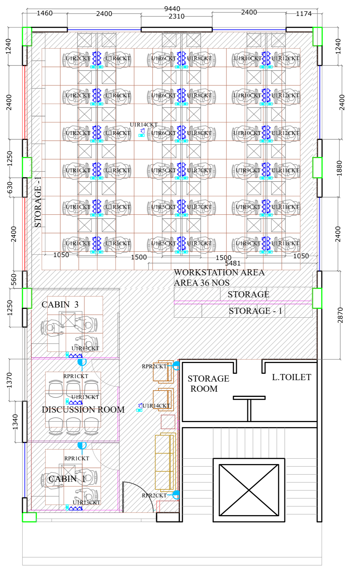
FIRST FLOOR POWER PLAN
