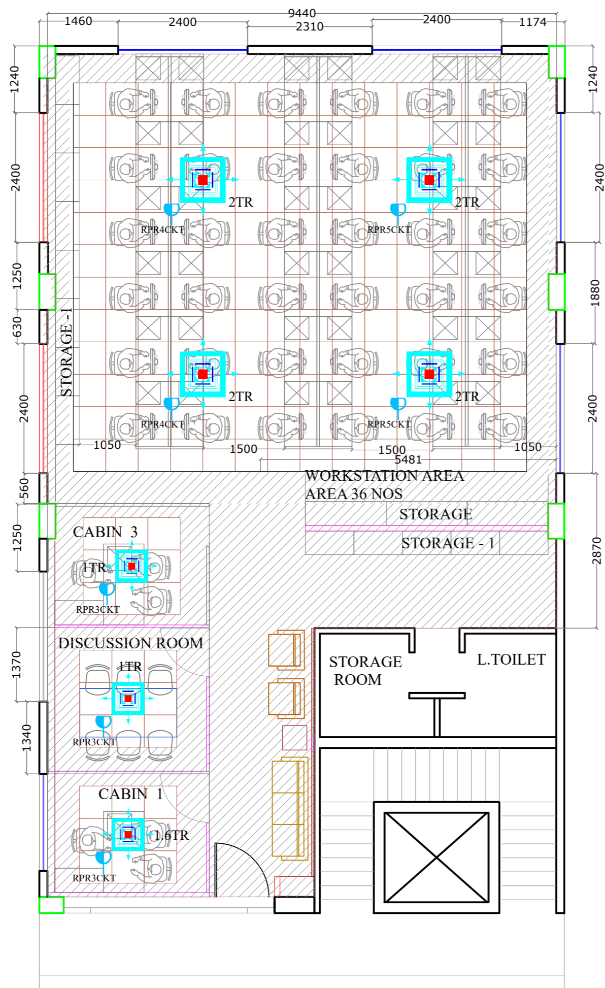
FIRST FLOOR AC PLAN
