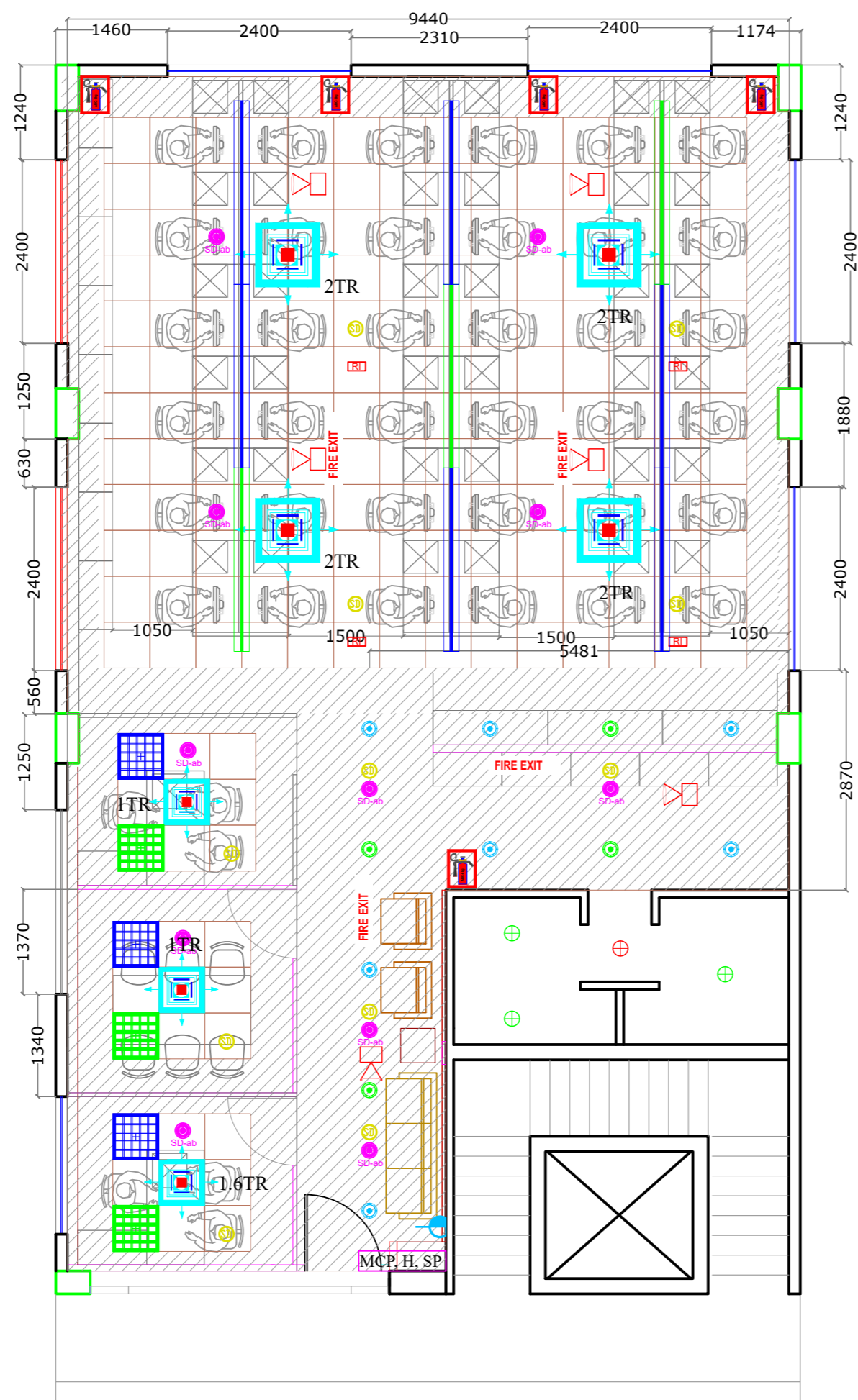
FIRST FLOOR FIRE ALARM, PUBLIC ADDRESS & ACCESS CONTROL PLAN
