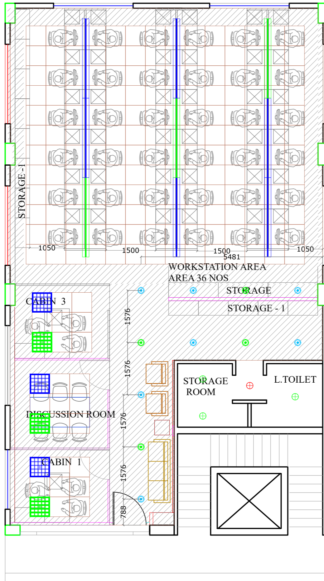
FIRST FLOOR LIGHTING PLAN
