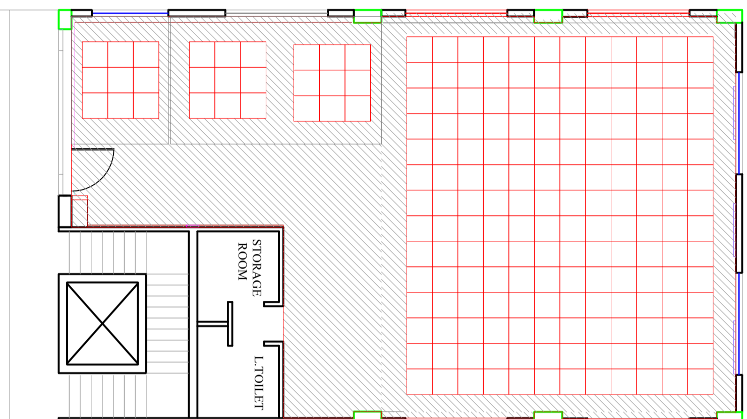
FIRST FLOOR PLAN OPTION -1
